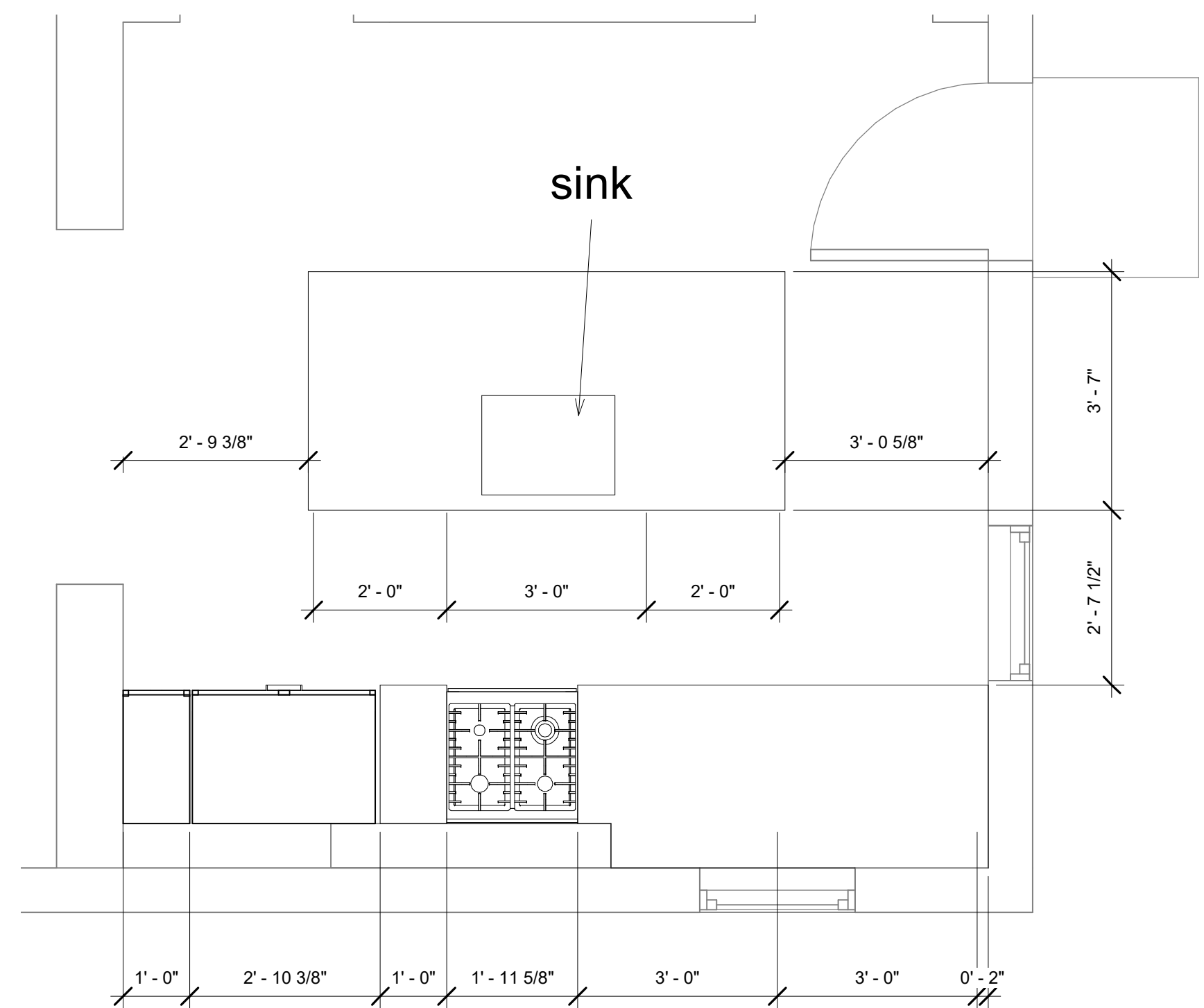
① First Floor Proposed Kitchen Callout 1 1/2" = 1'-0"
