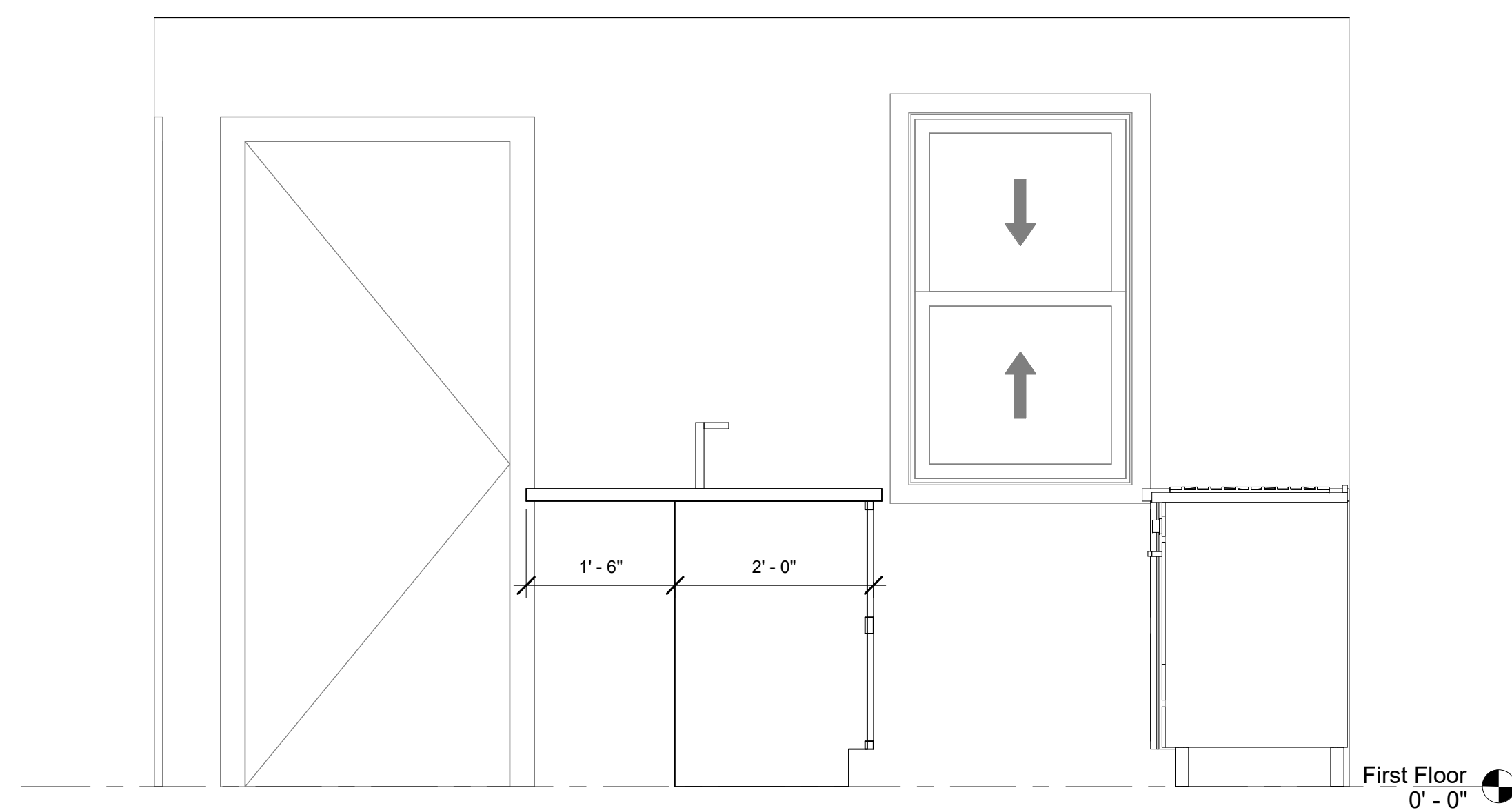
③ Kitchen East 3/4" = 1'-0"
