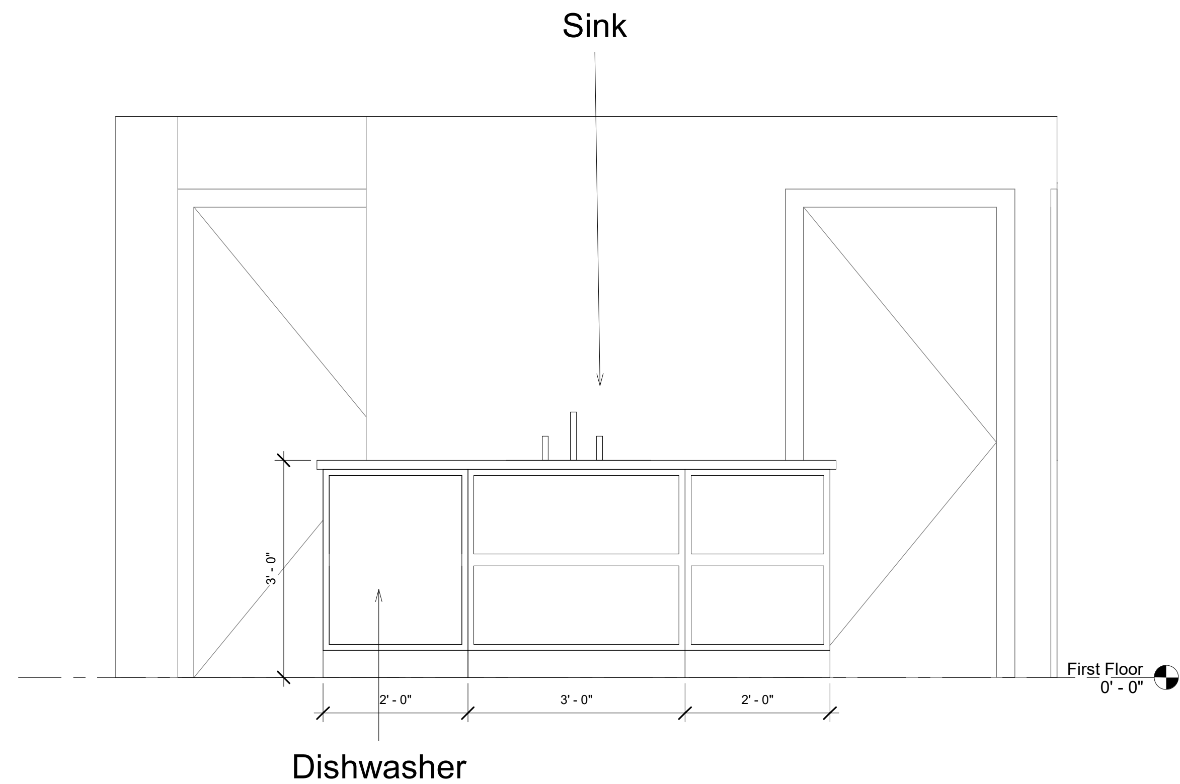
② Kitchen North 3/4" = 1'-0"
